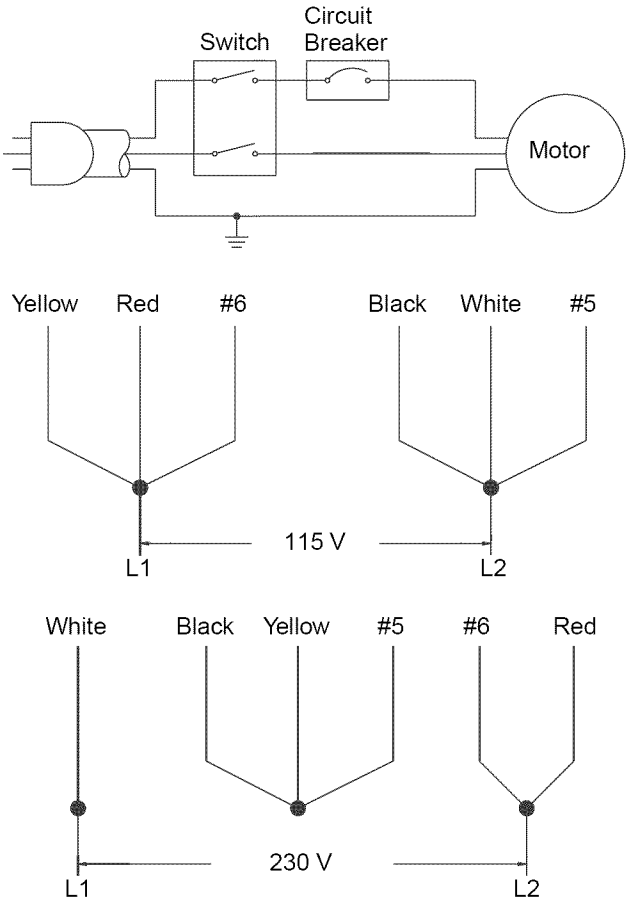
Figure 5 - Wiring Diagram
