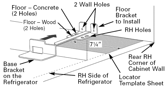
Figure 1 – Installation Overview
