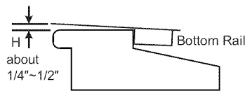
Wooden Window
