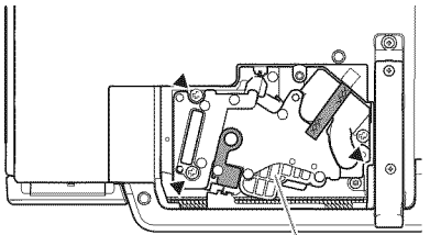
Lamp cartridge
