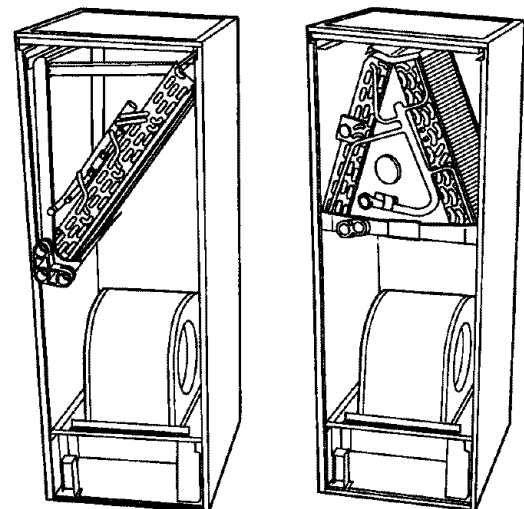
→ Fig. 3—Completed Downflow Conversion
