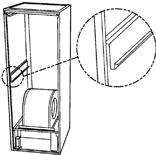
SLOPE COIL → Fig. 4—Downflow Slope Coil Bracket
