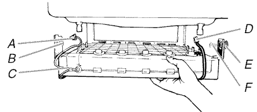
A. Cutter grid Harness D. Ice level sensor harness B. Screw E. Plastic spacer C. Cutter grid F. Screw
