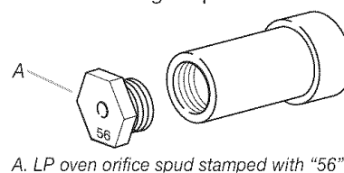
A. LP oven orifice spud stamped with "56"
