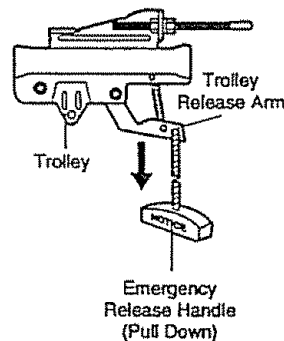
Manual disconnect position
