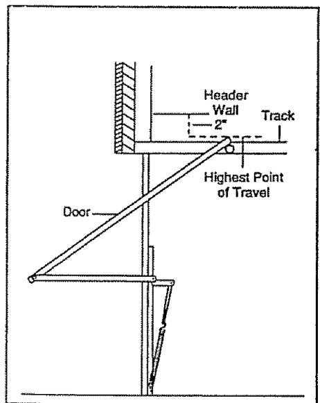
One-piece door with horizontal track
