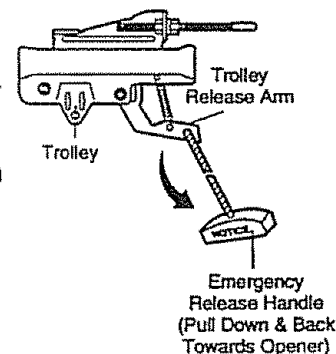
Lockout position
