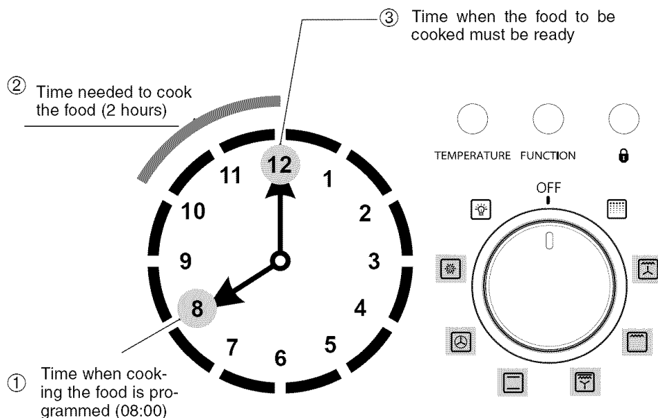
Programmable functions
