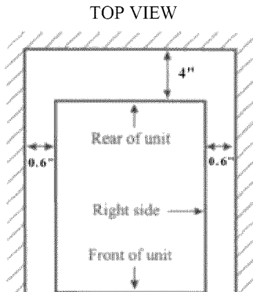
INSTALLATION CLEARANCES:
