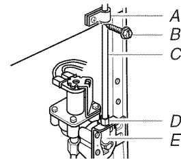
A. Tube clamp B. Tube clamp screw C. Copper tubing D. Compression nut E. Valve inlet
