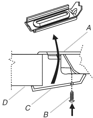
A. Cooktop B. Mounting screw C. Bracket B D. Countertop
