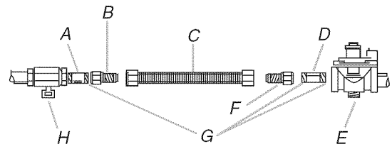
A. 3/8" nipple B. 3/8" adapter C. Flexible connector D. 3/8" nipple E. Gas pressure regulator F. 3/8" adapter G. Use pipe-joint compound. H. Manual gas shutoff valve
