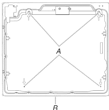
A. Mounting hole locations B. Front of cooktop
