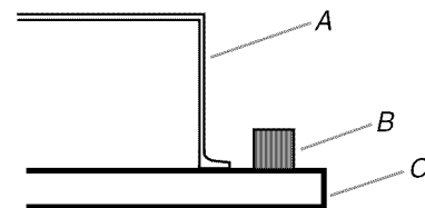
A. Burner box B. Foam strip C. Cooktop
