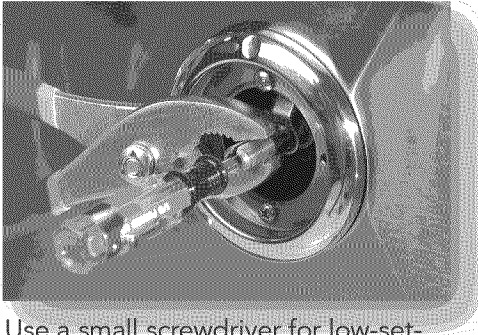
Use a small screwdriver for low-setting burner adjustment.
