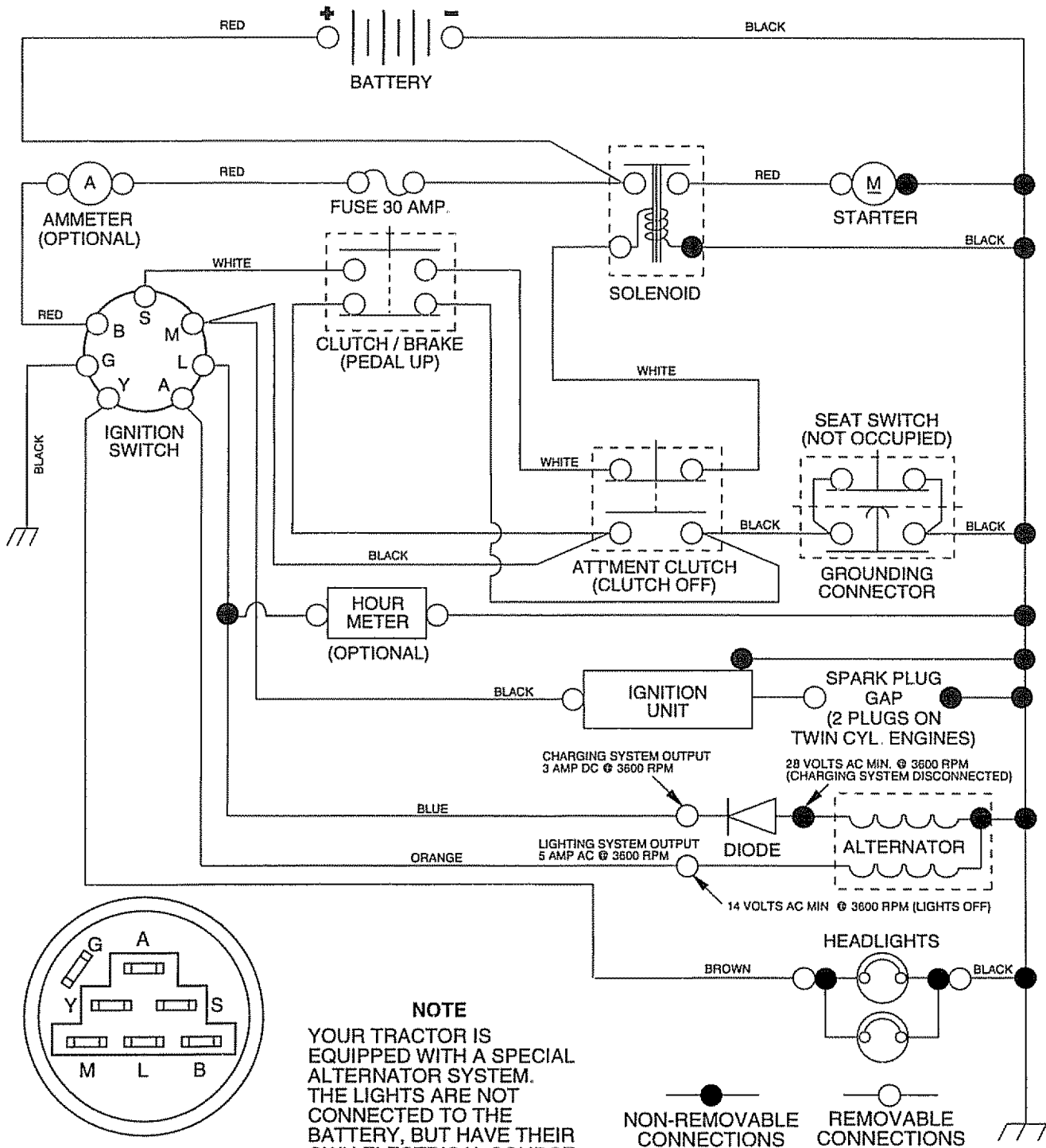
IGNITION SWITCH
