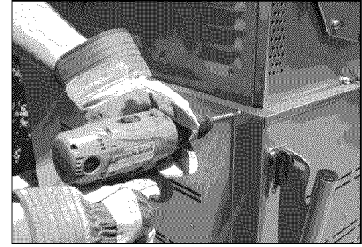
FIG. 12 Secure grill to rear of cart with (2) phillips-head screws provided (10-24 x 1/2").
