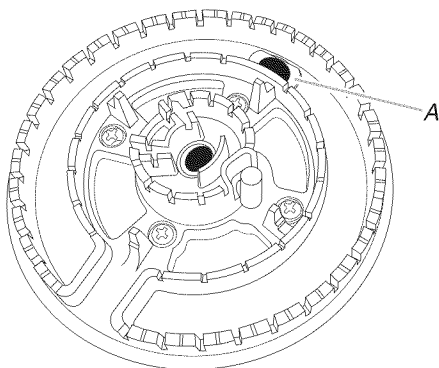
A. LP burner choke
