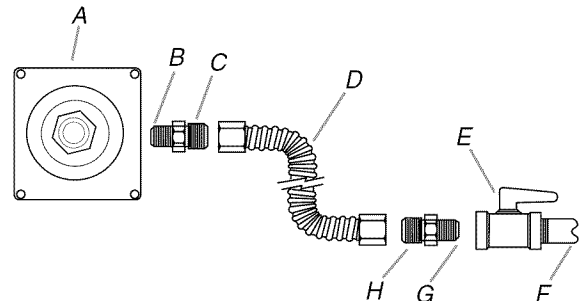
A. Gas pressure regulator B. Use pipe-joint compound. C. Adapter (must have ½" male pipe thread) D. Flexible connector
