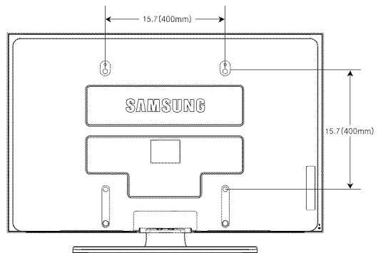
REAR VIEW
