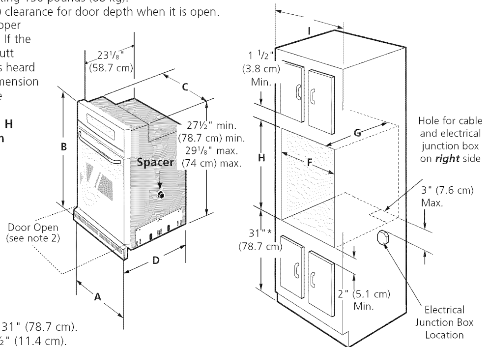
Figure 1 - SINGLE OVENS (Double Ovens see Figure 2)
