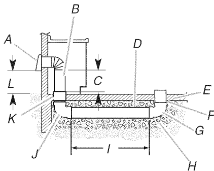
A. Wall cap B. 6" (15.2 cm) round metal vent C. 16" (40.6 cm) maximum D. 6" (15.2 cm) round PVC sewer pipe E. Concrete slab F. 6" (15.2 cm) round PVC sewer pipe G. 6" (15.2 cm) round 90° PVC sewer pipe elbow H. Tightly pack gravel or sand completely around pipe. I. 30 ft (9.1 m) max. J. 6" (15.2 cm) round 90° PVC sewer pipe elbow K. 6" (15.2 cm) round PVC coupling L. 12" (30.5 cm) minimum
