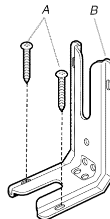
A. #12 x 1 3/8" screws B. Anti-tip bracket
