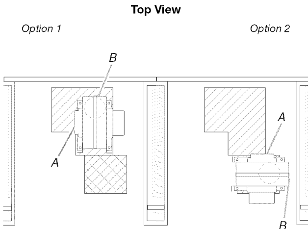
A. Inlet from range B. Exhaust outlet
