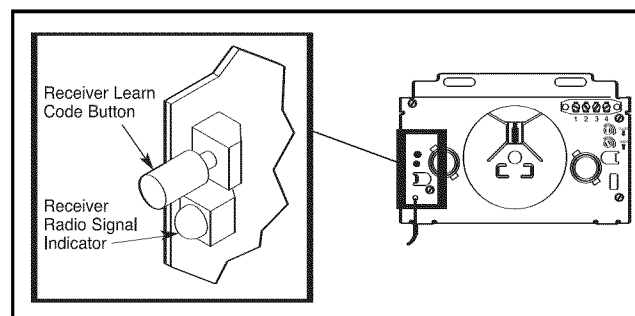
Figure 13 Learn Code Button and Indicator Light
