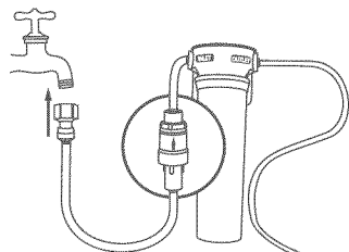
Fig.9 Connection to water supply
