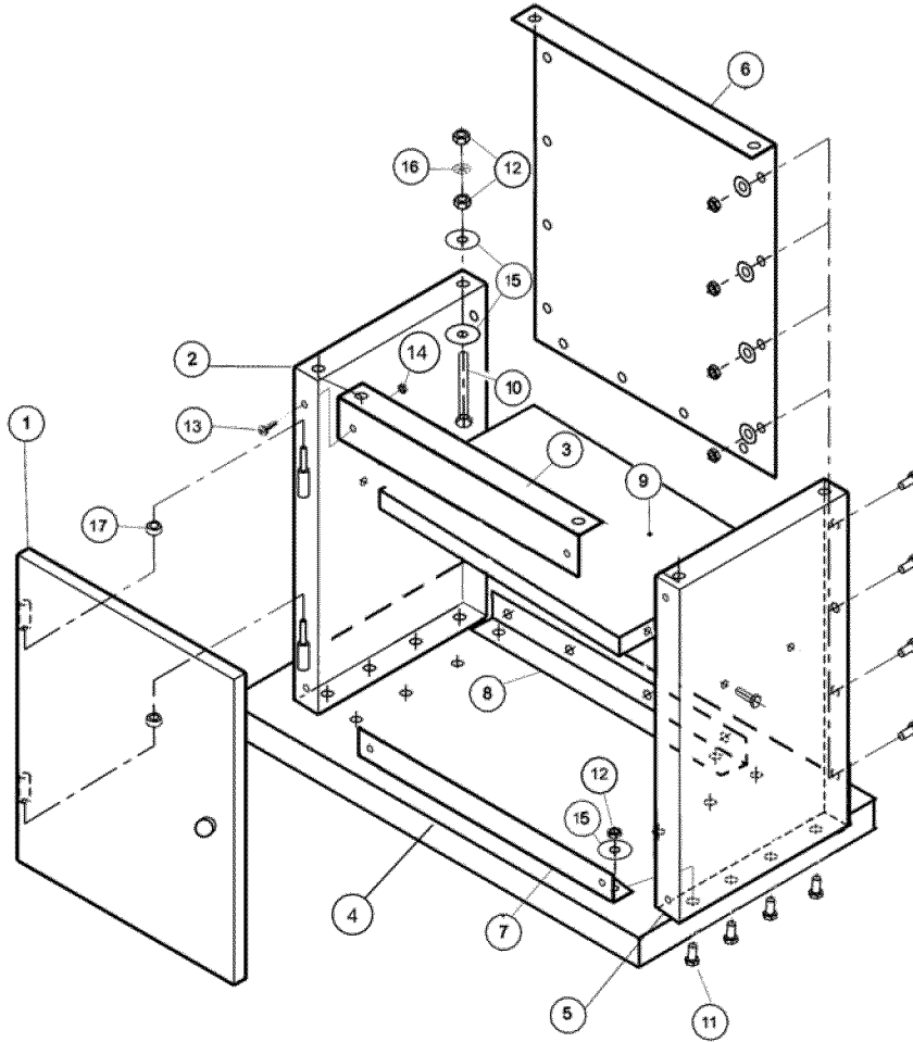
Figure 34 - Replacement Parts Illustration for Stand
