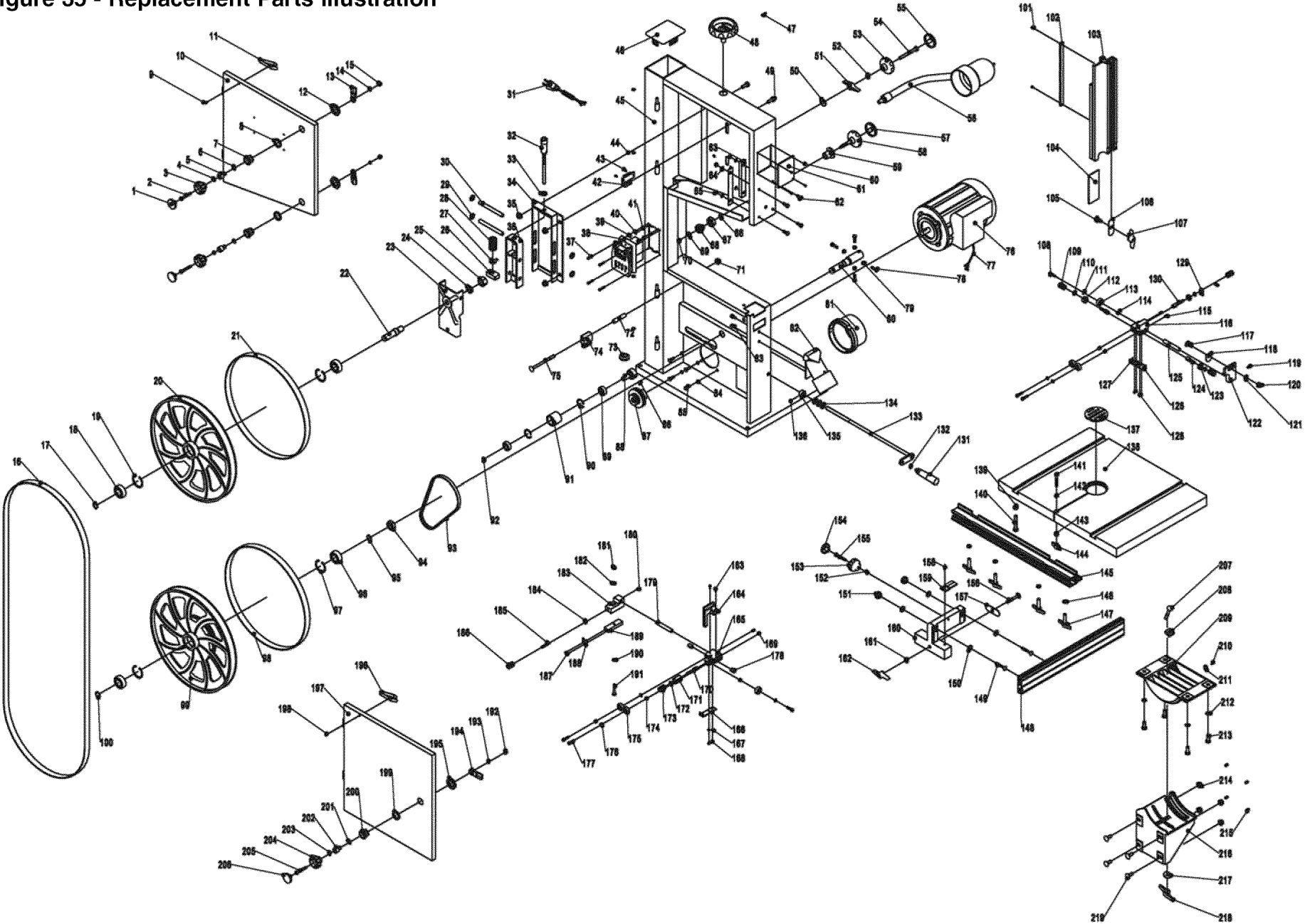
Figure 35 - Replacement Parts Illustration
