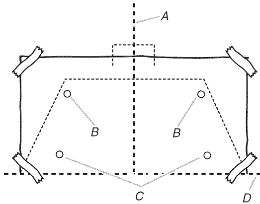
A. Centerline B. Upper screw locations C. Lower screw locations D. Mounting height reference
