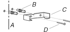
A. Centerline on wall B. 10 x 60 mm drywall anchors C. Vent cover bracket D. 6 x 70 mm screws
