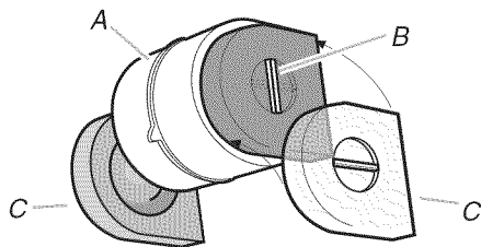
A. Blower housing B. Filter handle C. Charcoal filters
