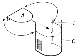
A. Deflector B. Upper screw holes C. Lower vent cover
