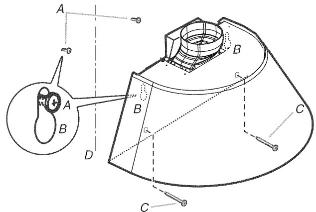
A. Mounting screws in upper screw locations B. Keyhole C. Mounting screws in lower screw locations D. Centerline on wall
