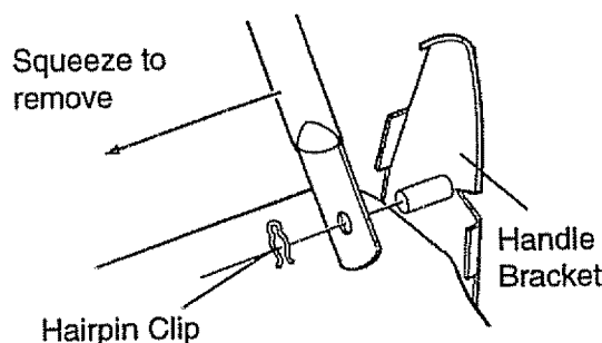
Lower Handle
