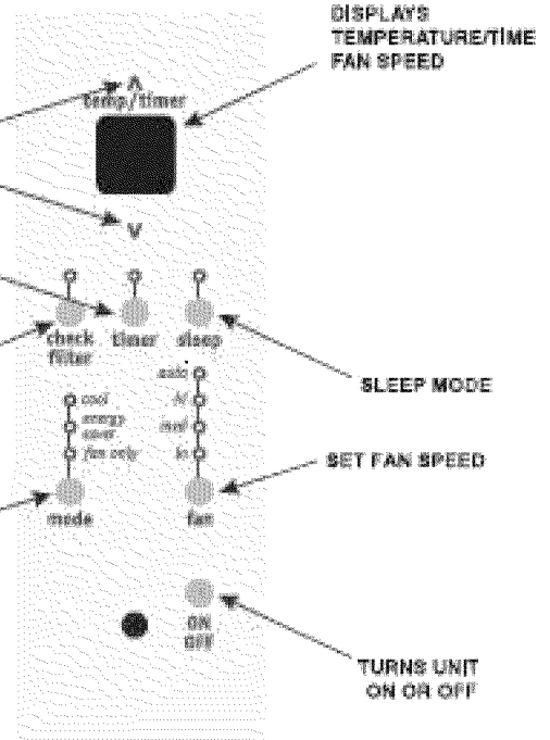
UNIT CONTROL
