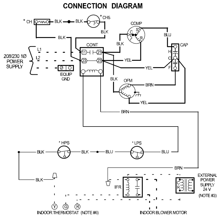
Fig. 7 - HC4A318-60 Typical Wiring Schematic
