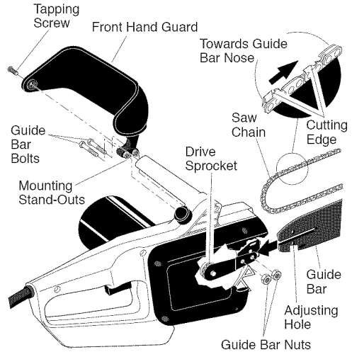
Figure 2 - Assembling Guide Bar, Chain, and Hand Guard
