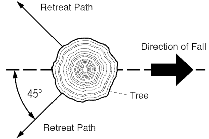
Figure 9 Retreat Path From Tree
