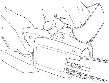
Figure 7 - Pressing Squeeze Bulb on Oil Cap to Oil Chain
