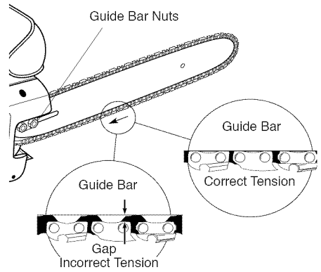
Figure 5- Saw Chain Adjustment
