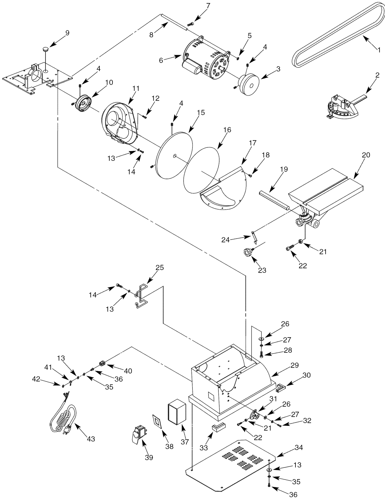
Figure 18 - Replacement Parts Illustration for Motor and Disc
