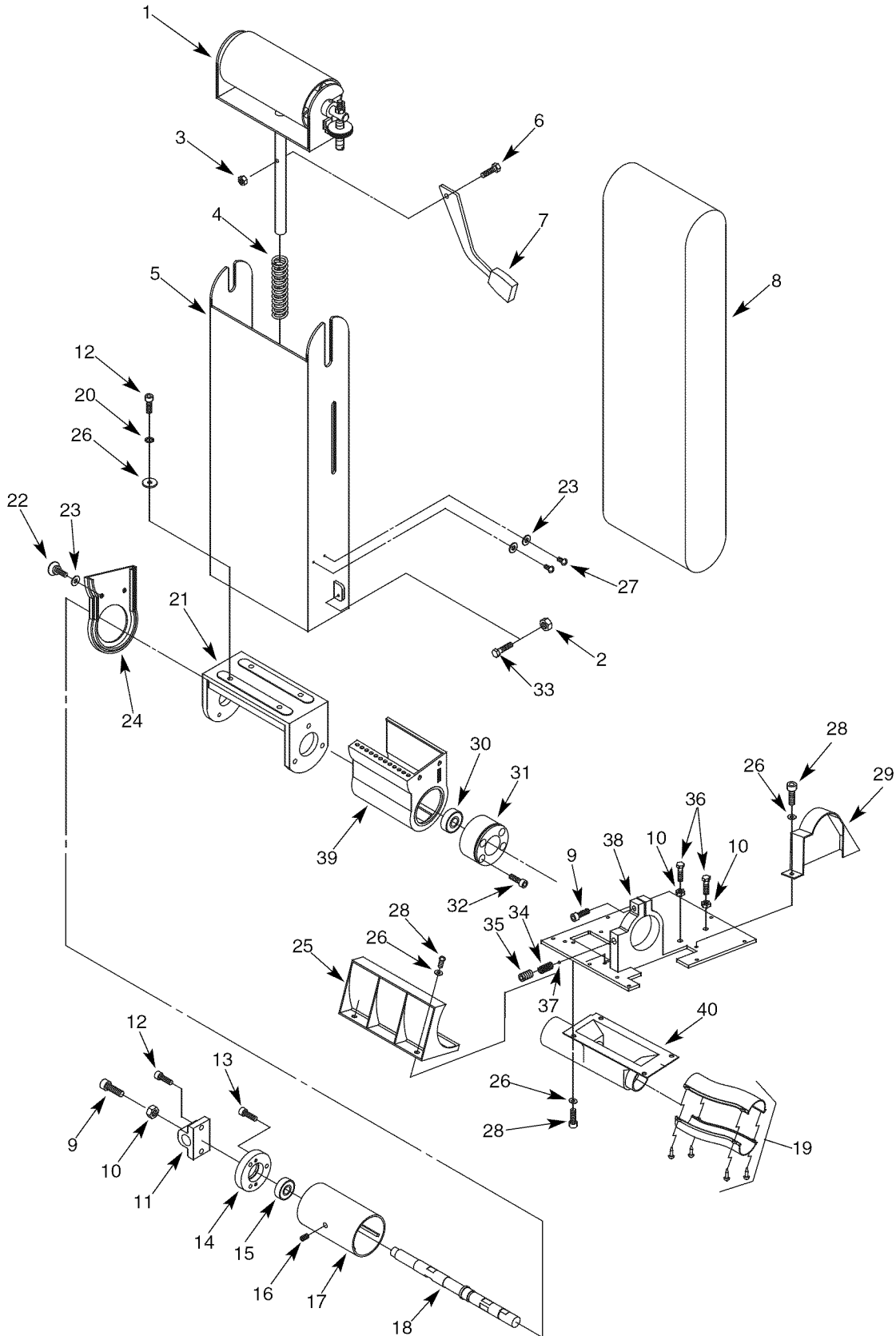
Figure 17 - Replacement Parts Illustration for Belt Housing
