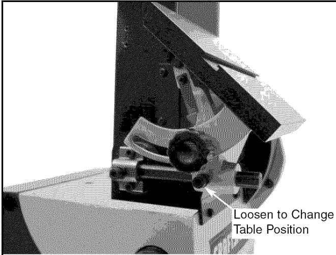
Figure 10 - Reposition Table when Tilting the Table
