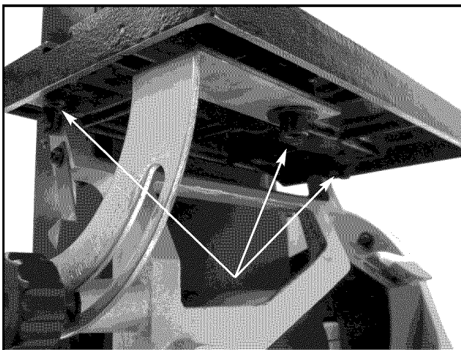
Figure 13 - Table Adjustment
