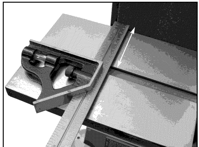
Figure 12 - Checking Parallelism of Table Slot to Belt
