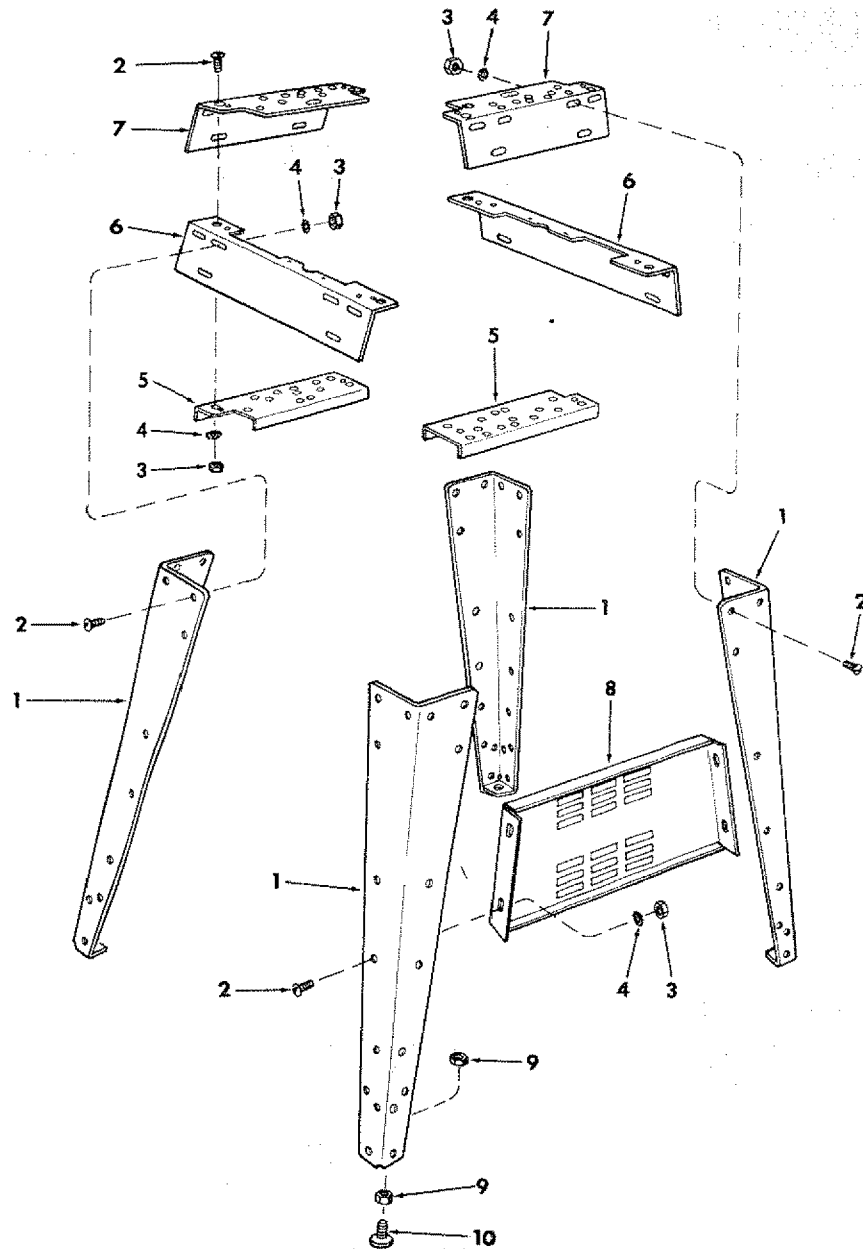
FIGURE 3 PARTS LIST SUPPLIED WITH MODEL 113.225831 ONLY
