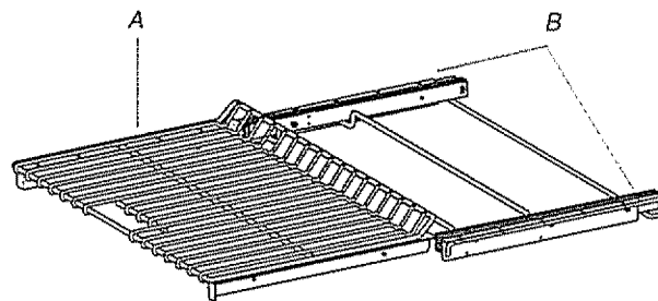
A. RollerGlide™ rack B. Sliding shelf
