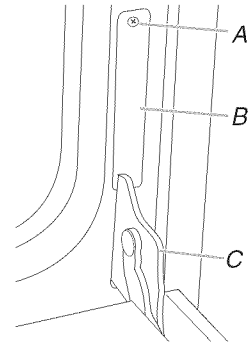
A. Hinge cover plate screw B. Hinge cover plate C. Hinge
