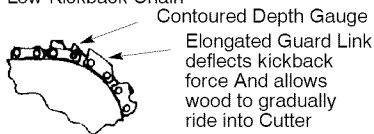
Low-Kickback Chain
