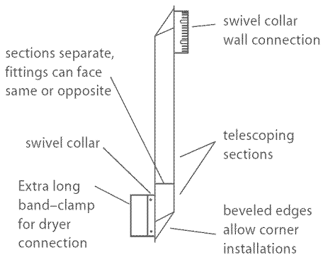
Fig.14 Installation configuration
