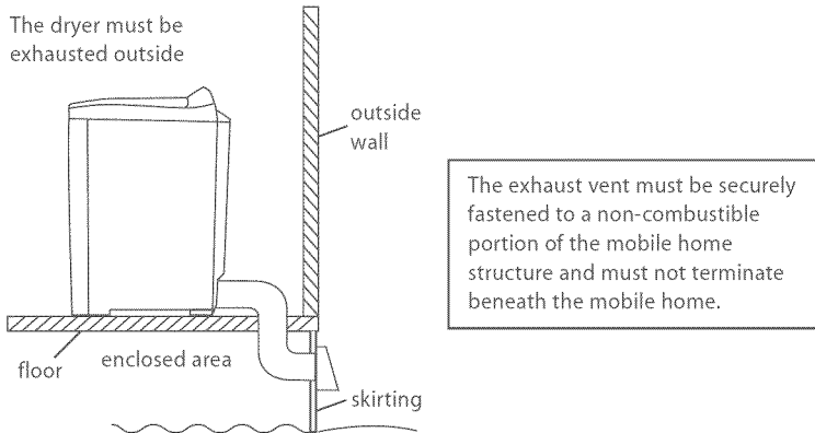
Fig.8 Exterior venting
