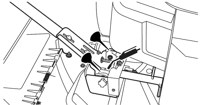
Figure 21. Lubricating Rider
