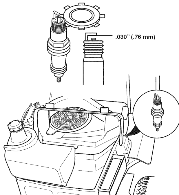
Figure 33. Spark Plug Gapping
