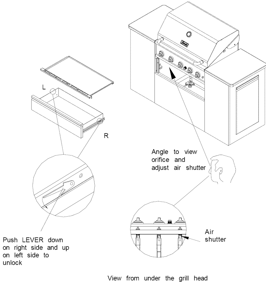
View from under the grill head
