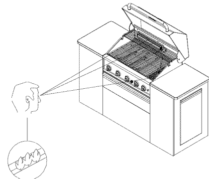
MAGNIFIED VIEW OF GRILL MAIN BURNER, INFRARED BURNER AND ROTISSERIE BURNER FLAME THROUGH OPEN LID.
