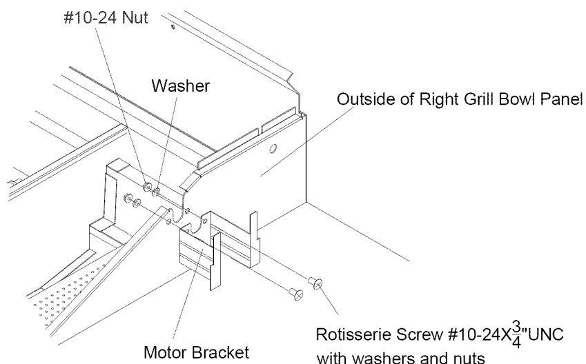
Rotisserie Screw #10-24x3/4" Qty. 2 Part # S112G10124
