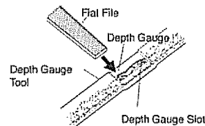
Figure 16 - Depth Gauge Tool On Chain
