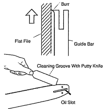
Figure 13 - Guide Bar Maintenance
