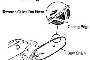
Figure 2 - Chain Position
