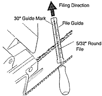
Figure 14 - File and File Guide Placement On Chain
