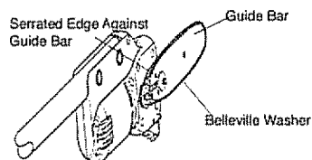
Figure 3 - Belleville Washer Assembly
