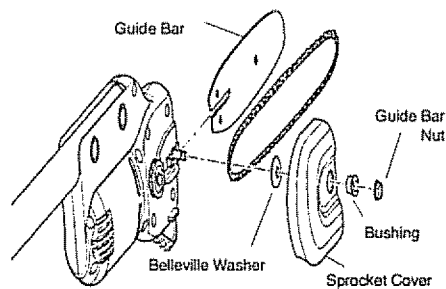
Figure 1 - Installing Guide Bar
