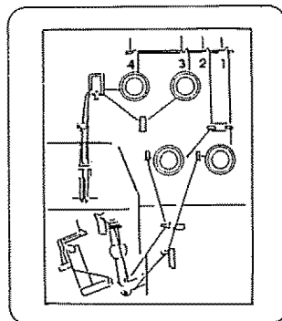
Threading Chart
