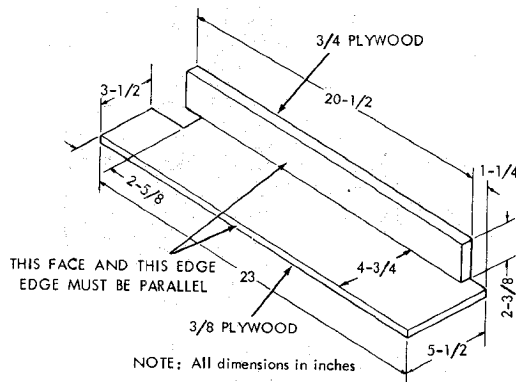
AUXILIARY FENCE
