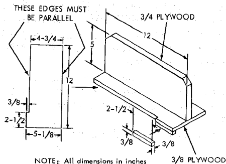
PUSH BLOCK
