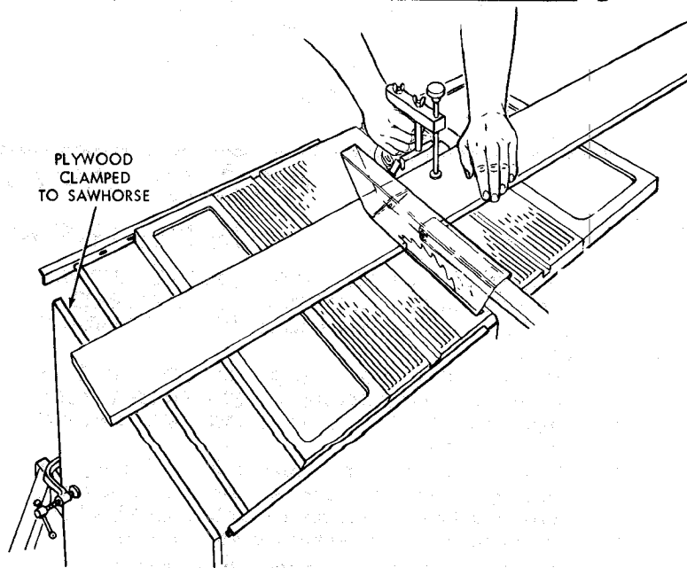
AUXILIARY FENCE
