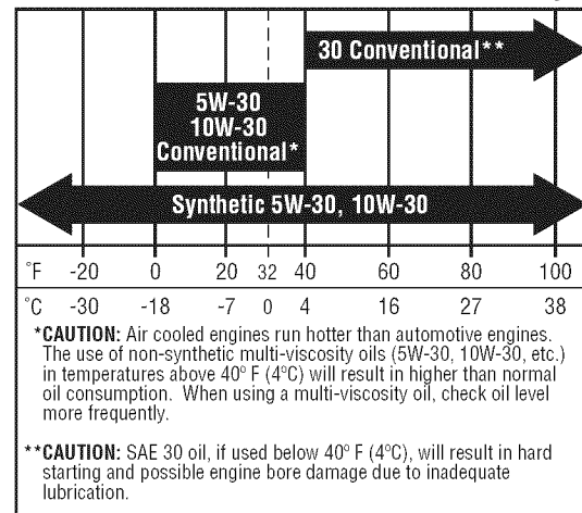
Figure 18. Recommended Engine Oil
