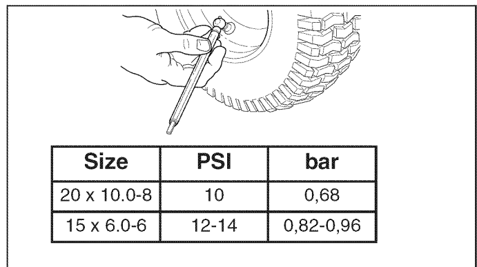
Figure 8. Tire Pressures
