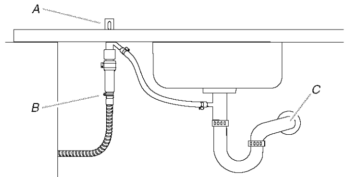
A. Drain hose connector B. Drain air gap C. Waste
