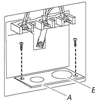
A. Small opening B. Large opening
