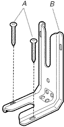
A. #12 x 1 1/2" screws B. Anti-tip bracket
