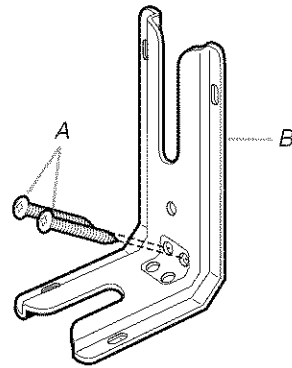
A. #12 x 1 1/2" screws B. Anti-tip bracket
