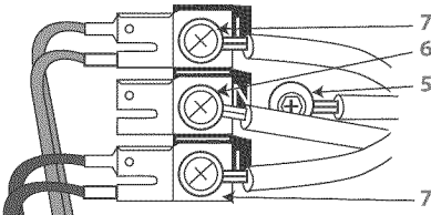
Fig.32 Connecting wiring
