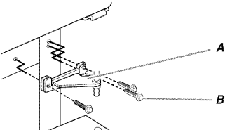
A. Center Hinge B. 5/16" Hex-Head Hinge Screws
