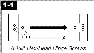
A. \frac{5}{16} " Hex-Head Hinge Screws
