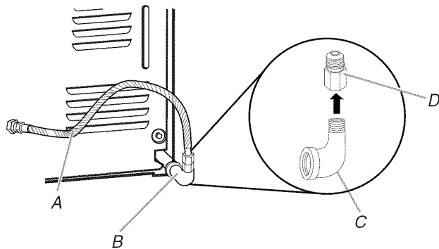
A. 3/8" flexible gas connector B. 3/8" dryer pipe C. 3/8" to 1/2" pipe elbow D. 1/2" pipe-to-flare adapter fitting
