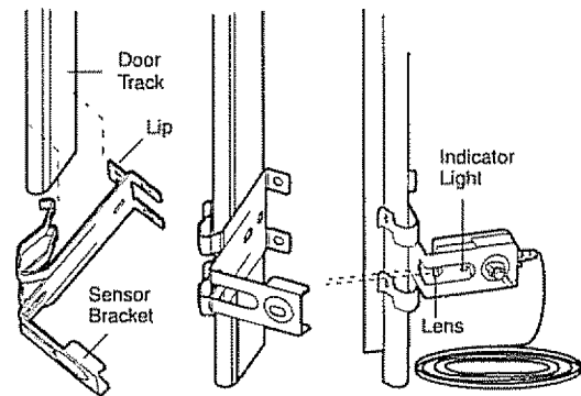
Figure 2 WALL MOUNT (RIGHT SIDE)
