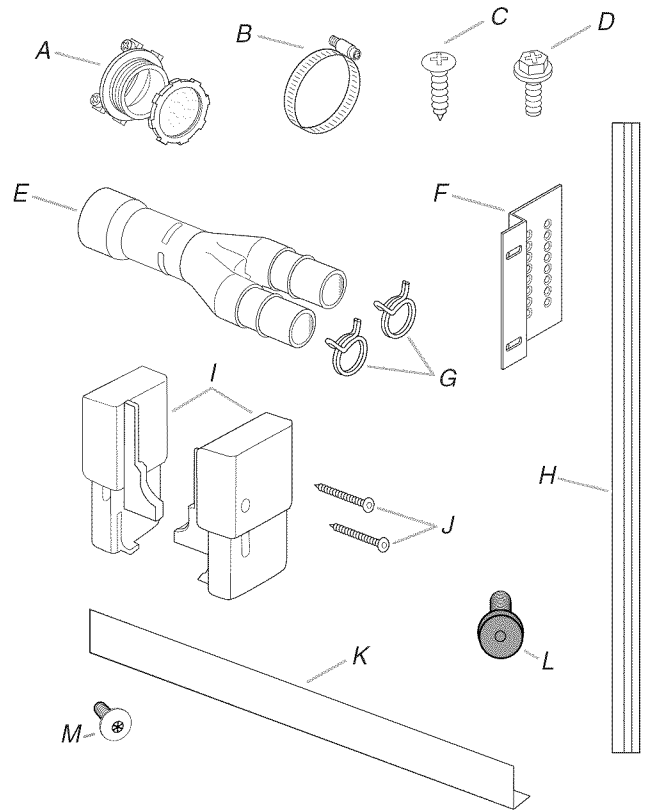
A. \frac{3}{4} " UL listed strain relief B. 1.25" hose clamp C. 8 mounting bracket screws D. 4 unit mounting screws E. Y drain connector F. 4 mounting brackets G. Drain connector spring clamps H. 2 trim strips I. Toe kick brackets J. 2 toe kick bracket screws K. Toe kick trim L. 2 panel fasteners (on some models) M. 10 TORX® screws (on some models)
