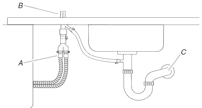
A. Drain hose connector B. Drain air gap C. Waste
