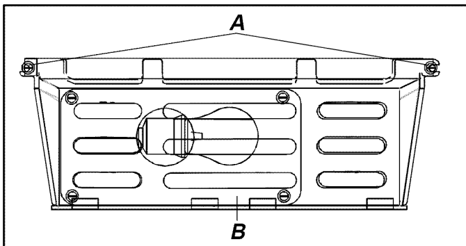
A ¼" hex nut screws B Light bulb cover
