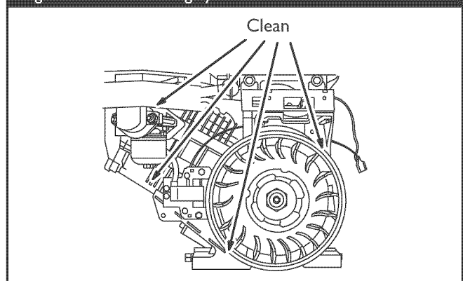
Figure 13 — Air Cooling System
