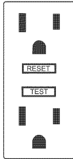
Figure 6 — 120 Volt, 15 Amp GFCI Duplex Receptacle
